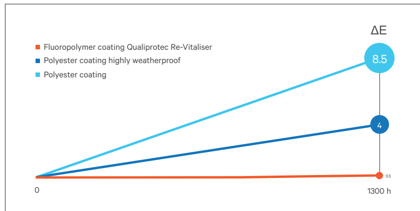
Florida test: minimal change in color ΔE Qualiprotec Re-Vitaliser (fluoropolymer technology) with best performance in direct comparison with other coatings
